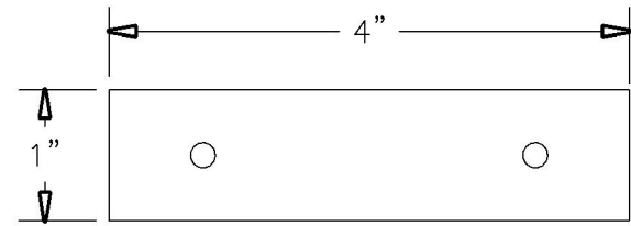
Handle X 2
