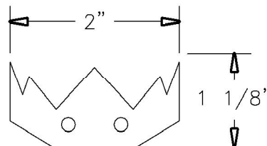
Guard X 2
